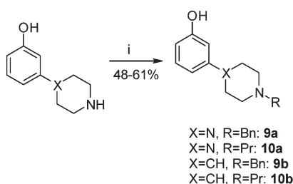
Scheme 2. Synthesis of Phenols 9a–10b a
