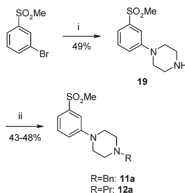
Scheme 3. Synthesis of Piperazines 11a and 12a a
