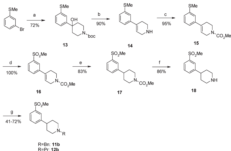
Scheme 1. Synthesis of Piperidines 11b and 12b a
